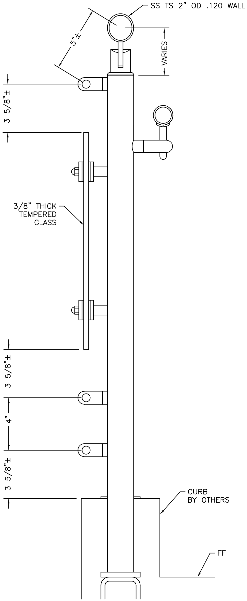
SECTION TOP-MOUNT OLYMPIAN RAIL WITH ROD LATERALS
