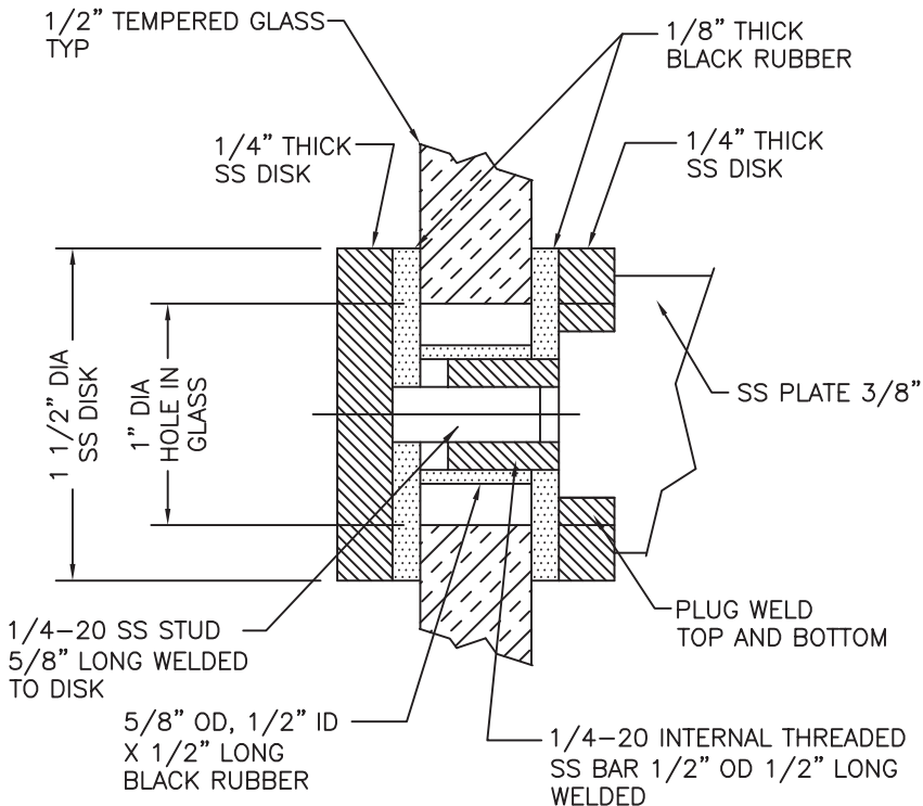
SECTION HANDRAIL BRACKET CONNECTION
