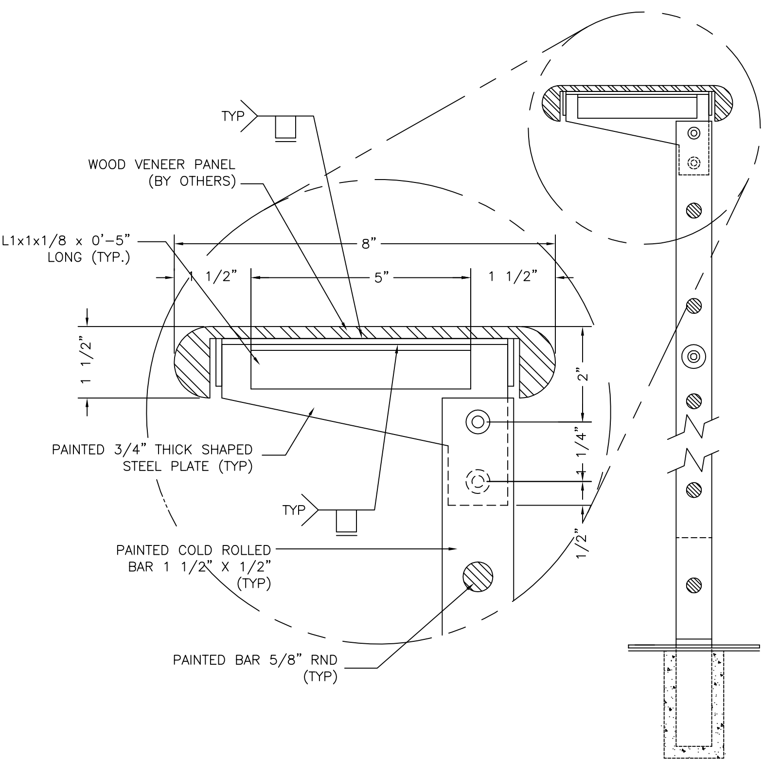
SECTION FABRICATED STEEL RAIL
