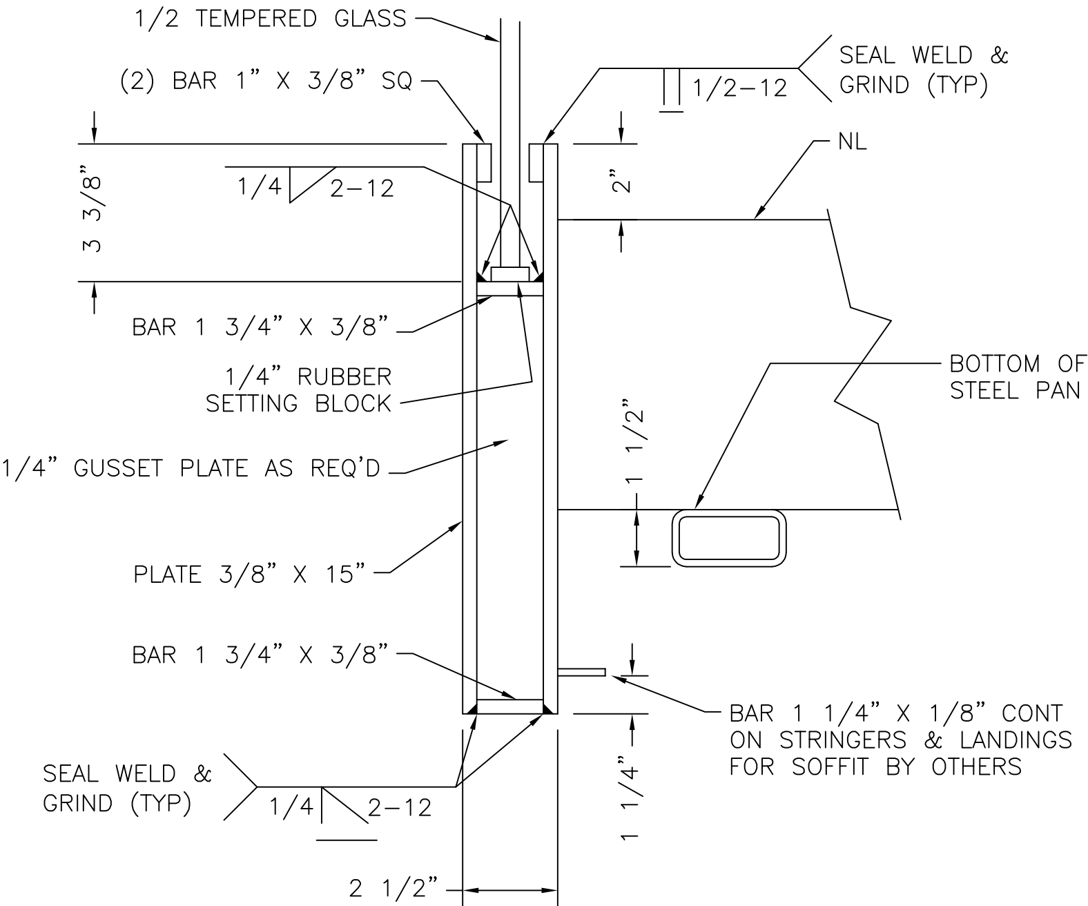
SECTION FABRICATED BOX STRINGER WITH INTEGRAL SHOE
