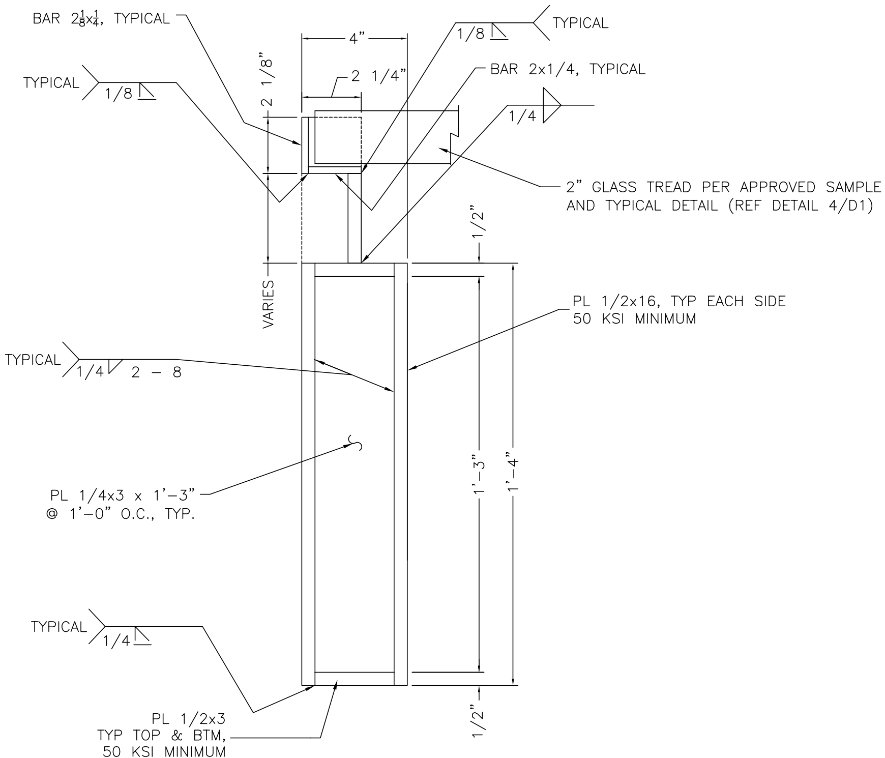
SECTION FABRICATED BOX STRINGER
