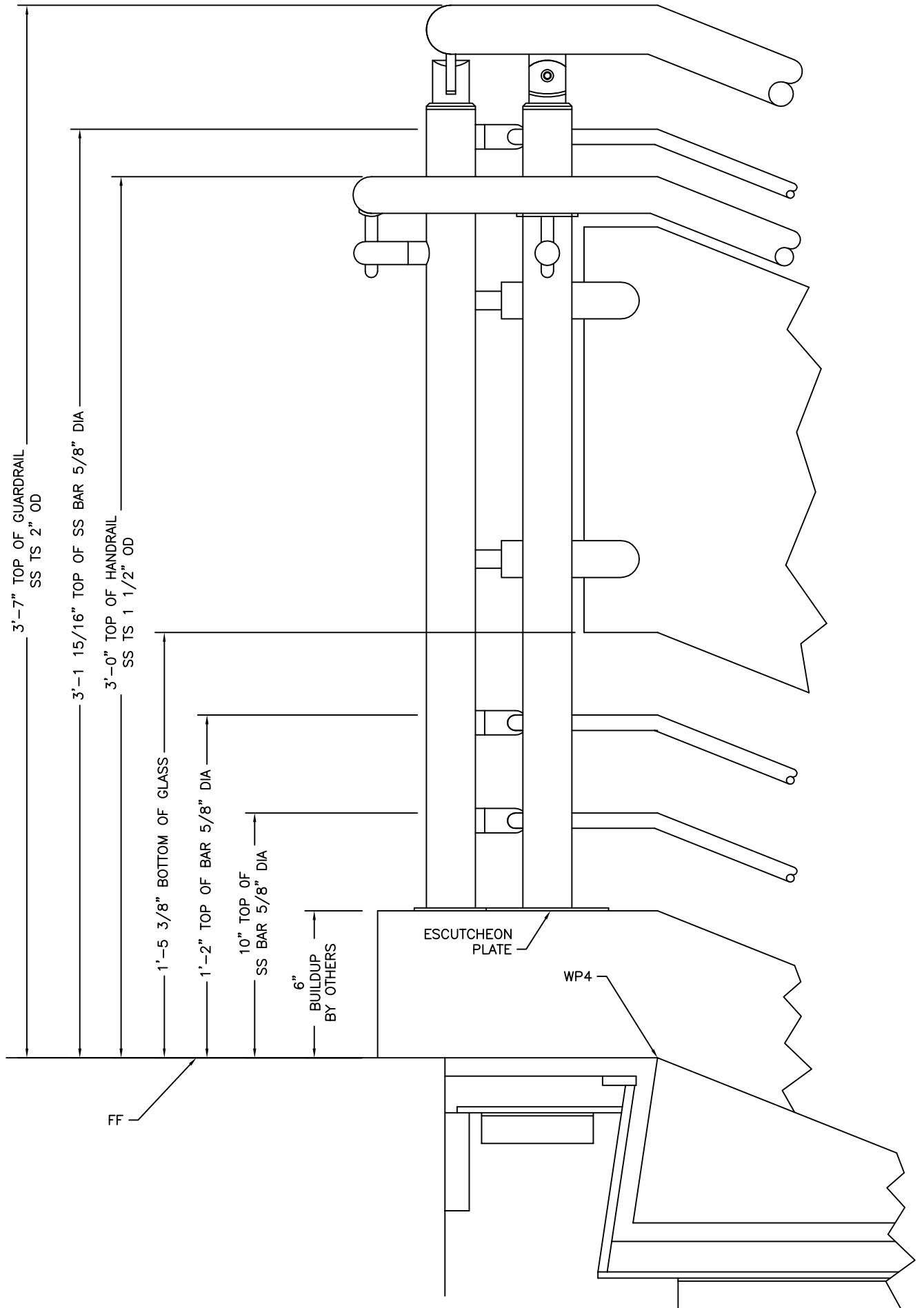
ELEVATION TOP-MOUNT OLYMPIAN RAIL WITH ROD LATERALS
