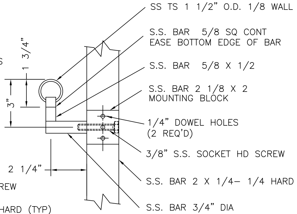
DETAILS GIBRALTAR RAIL
