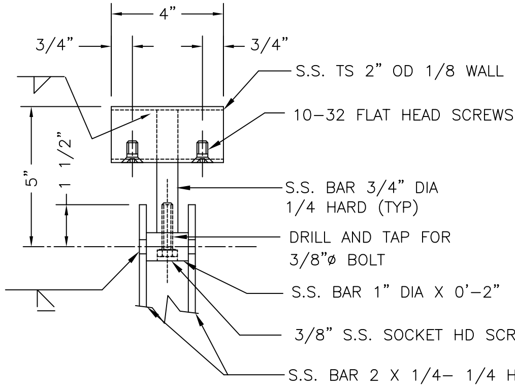
DETAILS GIBRALTAR RAIL
