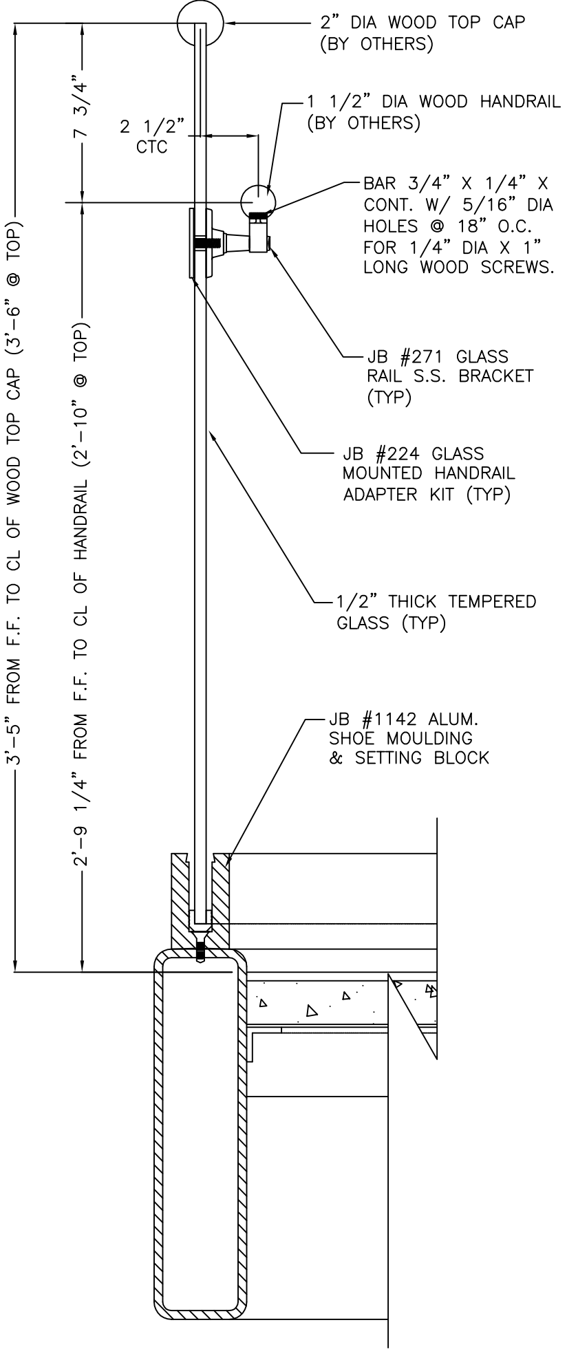
SECTION GLASS RAIL IN STANDARD ALUMINUM SHOE
