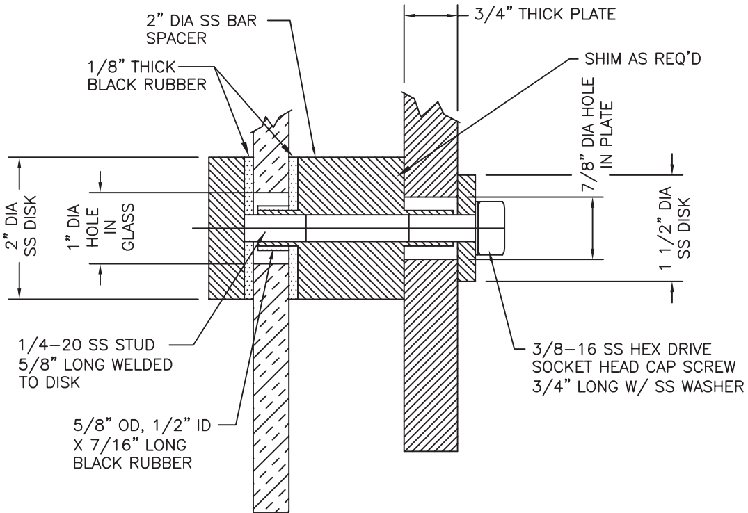
SECTION GLASS PIN OR "BUTTON" MOUNT
