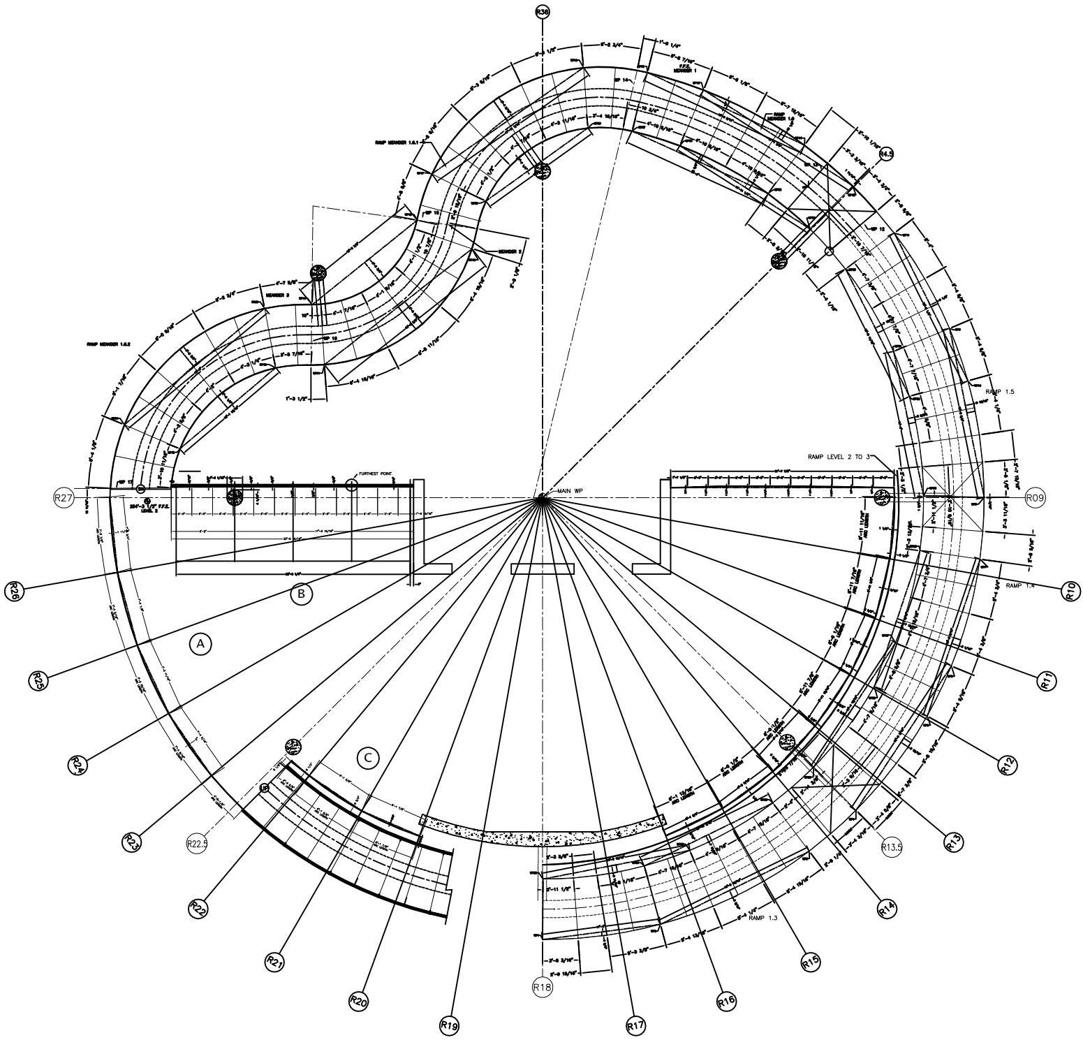
PLAN LAYOUT OF FABRICATED STEEL RAIL
