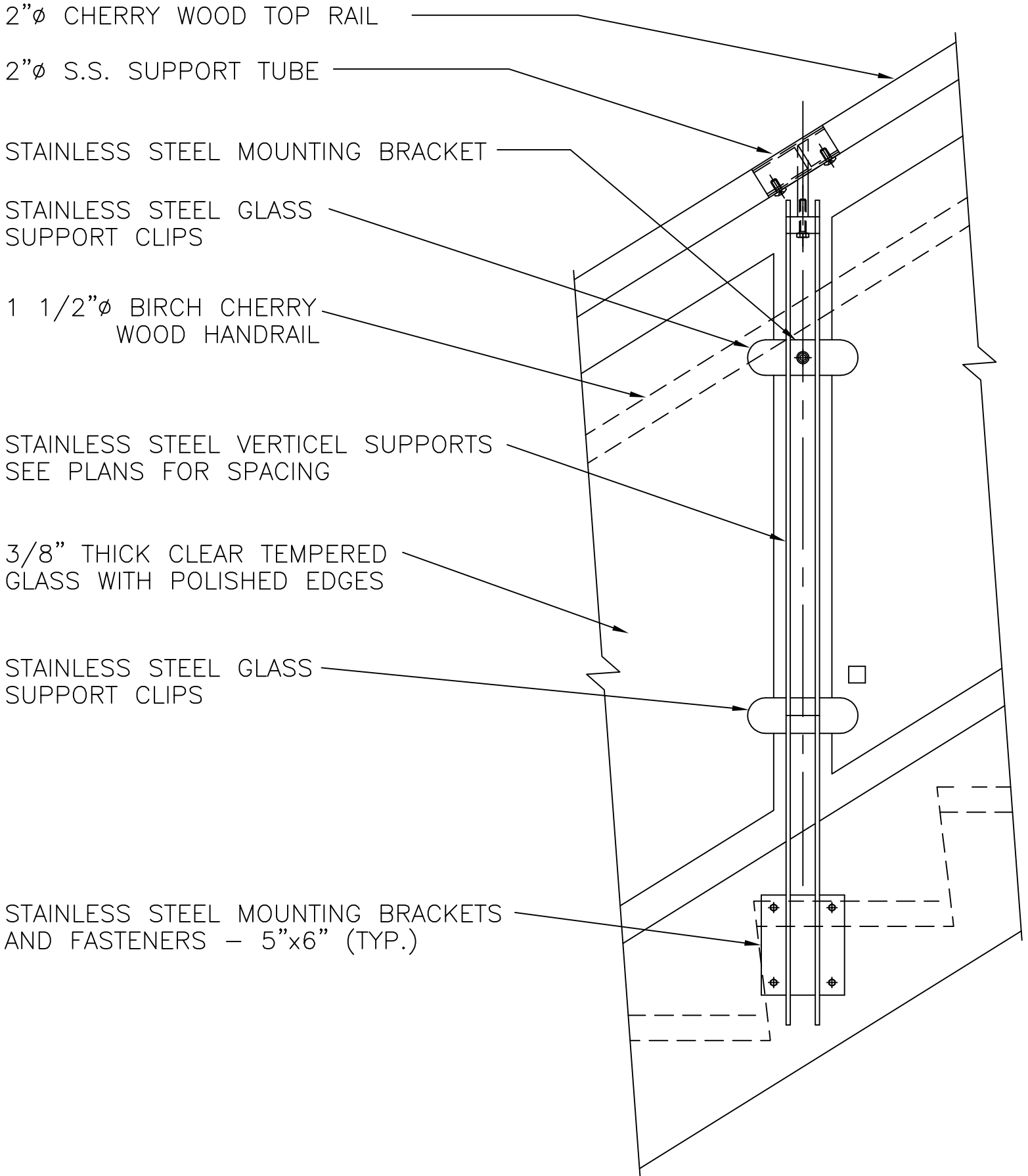
ELEVATION SIDE-MOUNT GIBRALTAR RAIL
